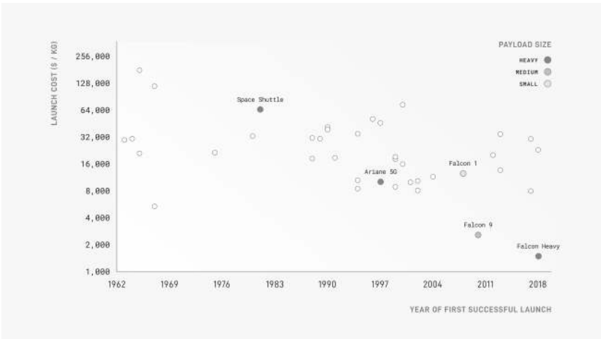
Cost of Space Launches to Low-Earth Orbit (constant 2021 $ per kilogram; plotted on a logarithmic axis)
